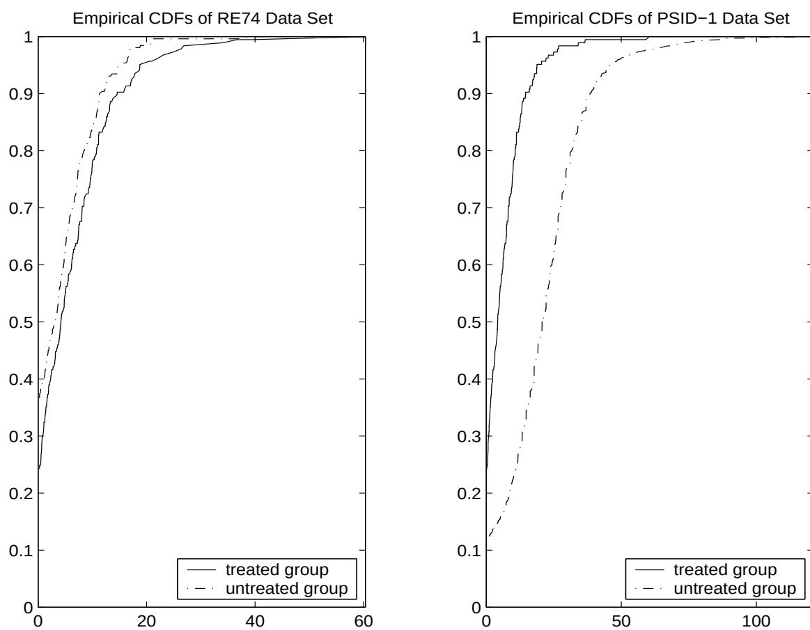
Figure 1: Empirical CDFs of RE74 and PSID-1 data sets
