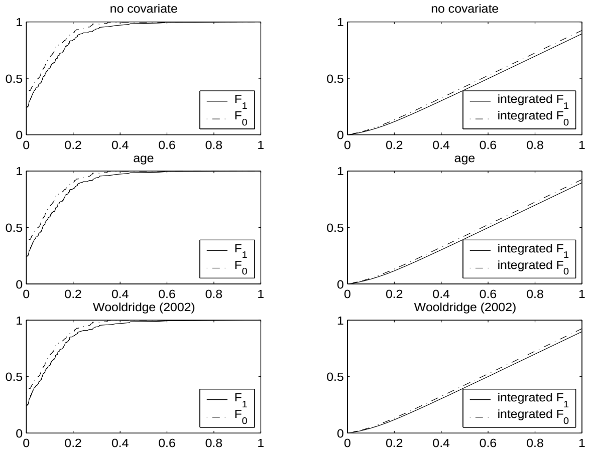
Figure 2: Estimated CDFs and Integrated CDFs for RE74 under Different Specifications.
