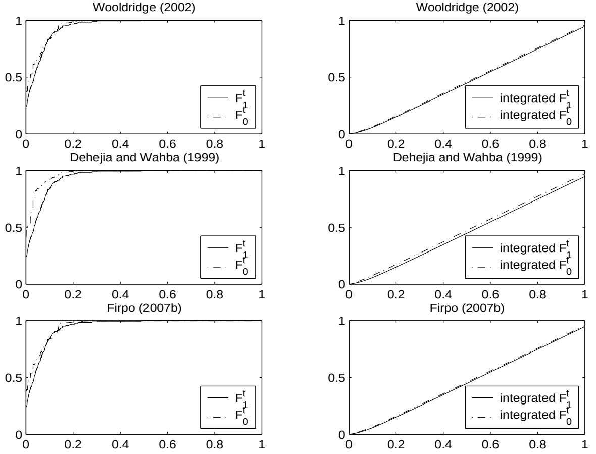
Figure 3: Estimated F_i^t 's and Integrated F_i^t 's for PSID-1 under Different Specifications.
