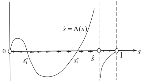
Figure 3 Sink Balanced Growth Path s_1^* : \Sigma \in \Sigma_{21}
