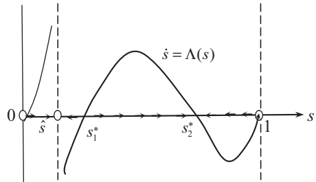
Figure 5 Sink Balanced Growth Path s_2^* : \Sigma \in \Sigma_{22}
