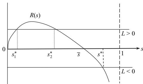
Figure 1 Existence of Balanced Growth Paths in General Fund Financing Taxes
