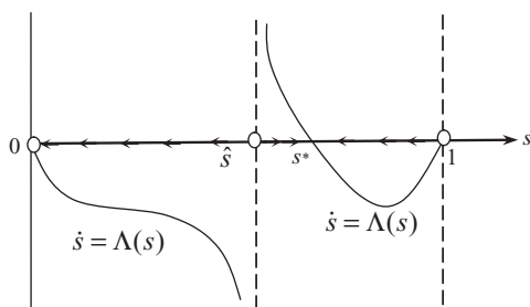
Figure 2 Unique Sink Balanced Growth Path: \Sigma \in \Sigma_{12} .
