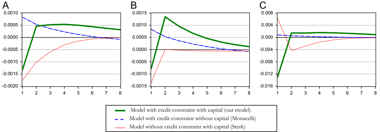
Fig. 2. Impulse responses of aggregate output, employment and consumption to monetary tightening. Note: The horizontal axis is divided in quarters; the vertical axis represents percentage deviations from a steady state. (A) Aggregate output, (B) Aggregate employment, (C) Aggregate consumption.
