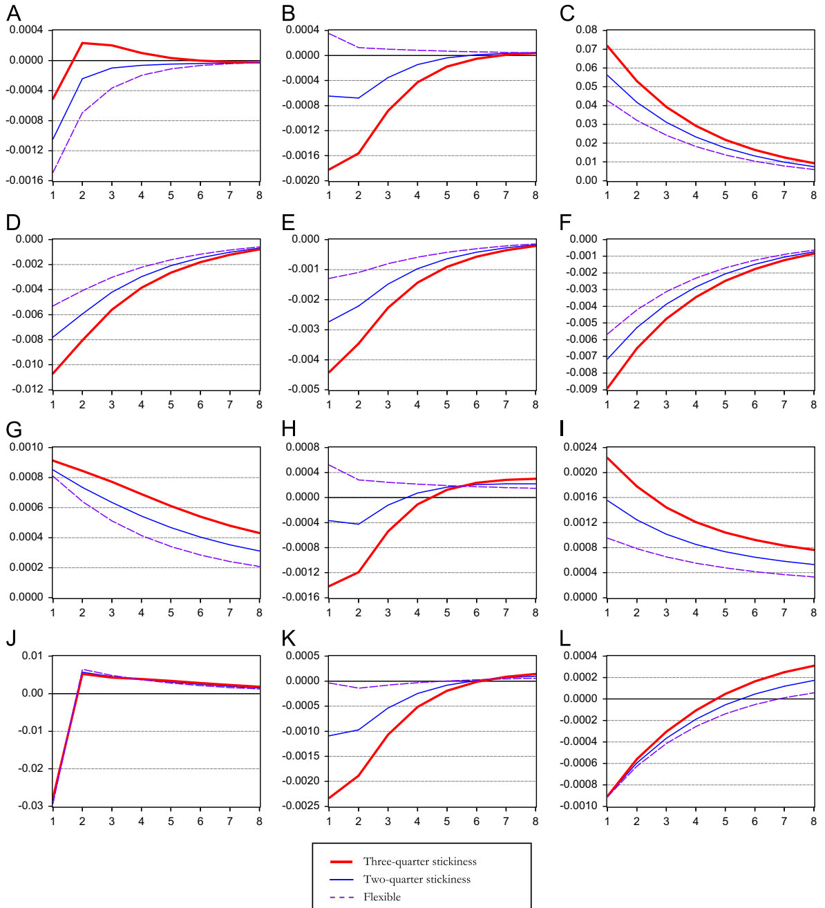
Fig. 3. Sensitivity analysis: impulse responses with decreasing degrees of nondurable price stickiness. Note: The horizontal axis is divided in quarters; the vertical axis represents percentage deviations from a steady state. (A) Nominal interest rate, (B) Relative price of durables, (C) Shadow price of borrowing, (D) Real debt, (E) Borrower's non-durable consumption, (F) Borrower's durable services, (G) Capital stock, (H) Saver's non-durable consumption, (I) Saver's durable services, (J) Aggregate real profits, (K) Aggregate non-durable consumption, (L) Aggregate durable services.
