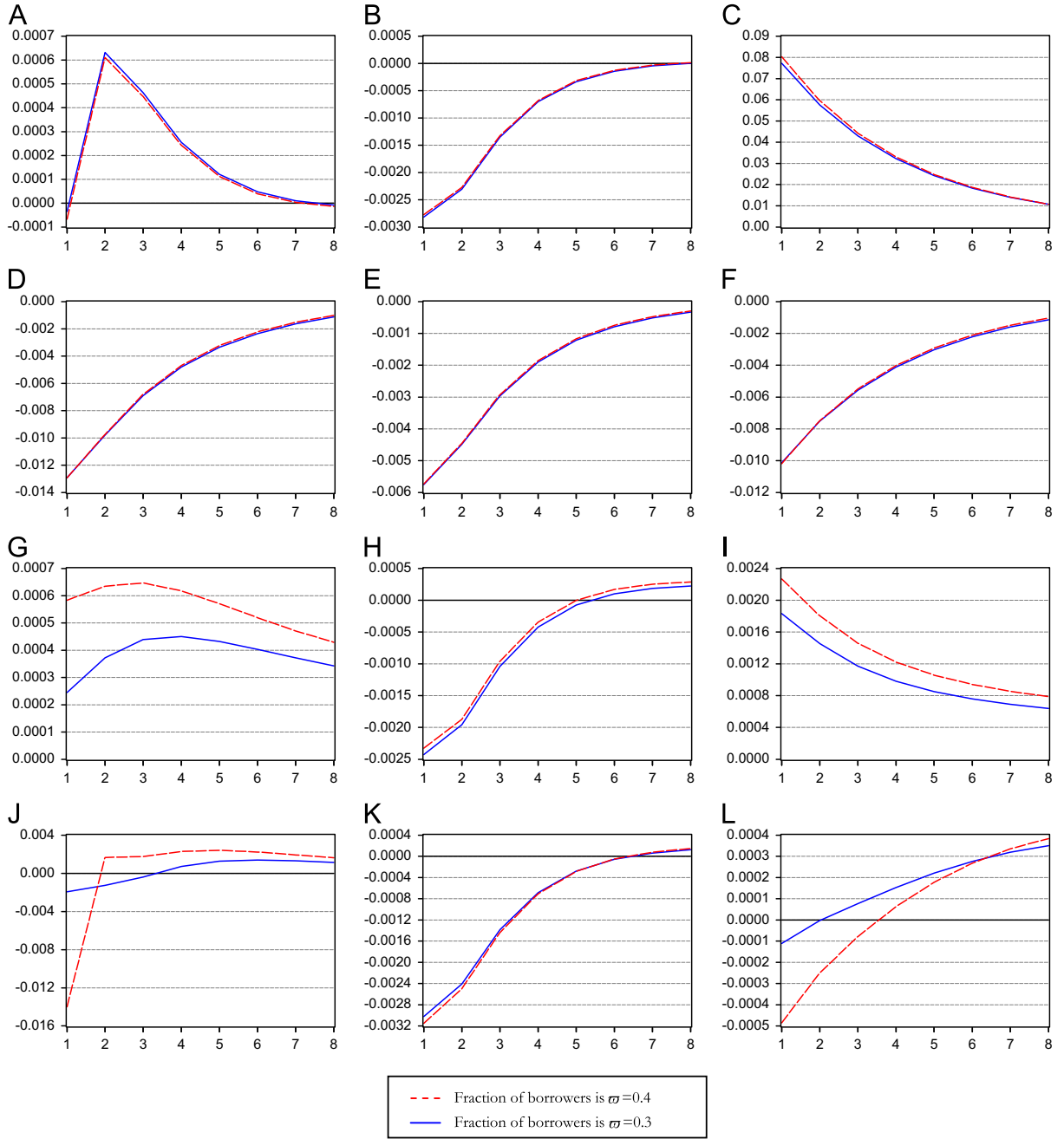
Fig. 4. Sensitivity analysis: impulse responses with decreasing fractions of borrowers. Note: The horizontal axis is divided in quarters; the vertical axis represents percentage deviations from a steady state. (A) Nominal interest rate, (B) Relative price of durables, (C) Shadow price of borrowing, (D) Real debt, (E) Borrower's non-durable consumption, (F) Borrower's durable services, (G) Capital stock, (H) Saver's non-durable consumption, (I) Saver's durable services, (J) Aggregate real profits, (K) Aggregate non-durable consumption, (L) Aggregate durable services.
