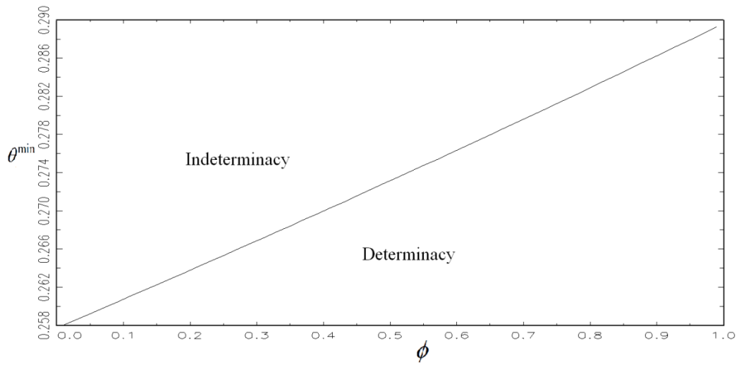
Figure 1. \theta^{\min} as a function of \phi .
